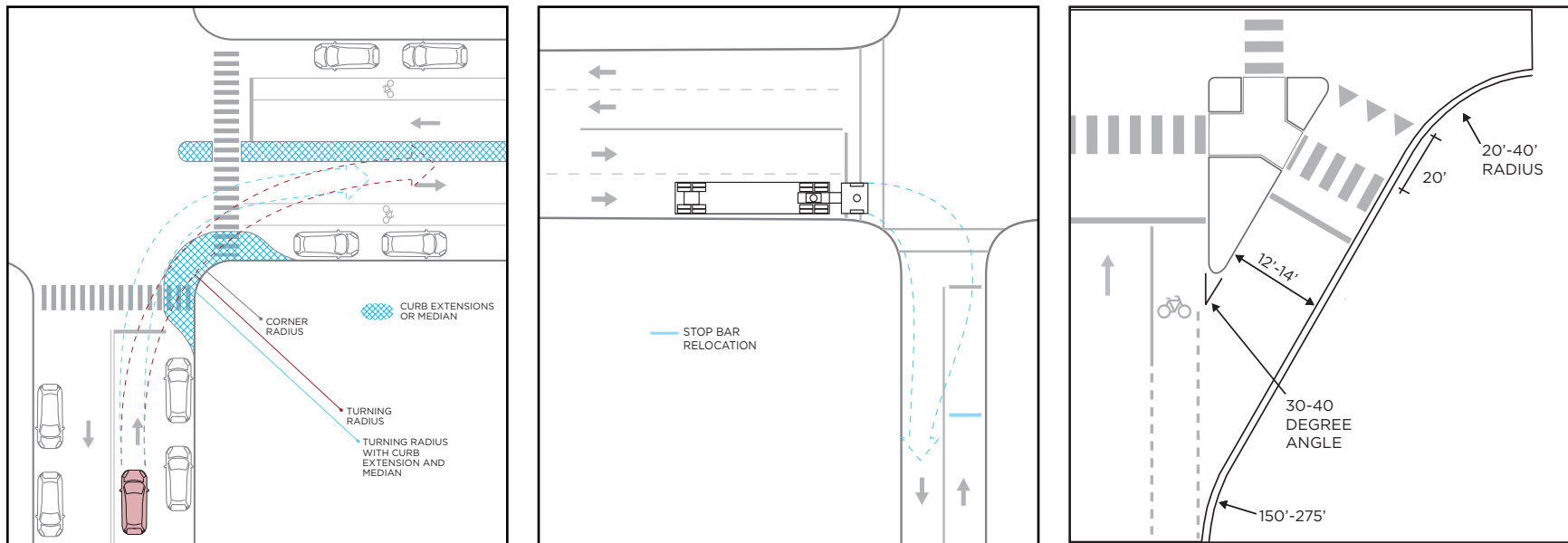
Corner Design Concepts
