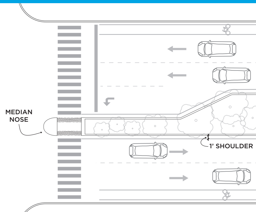
Crosswalk and Turn Lane at Median
