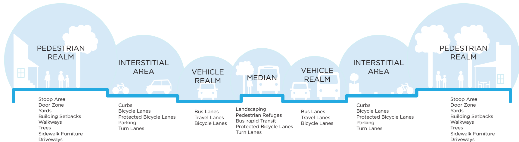
Cross-Section Elements
