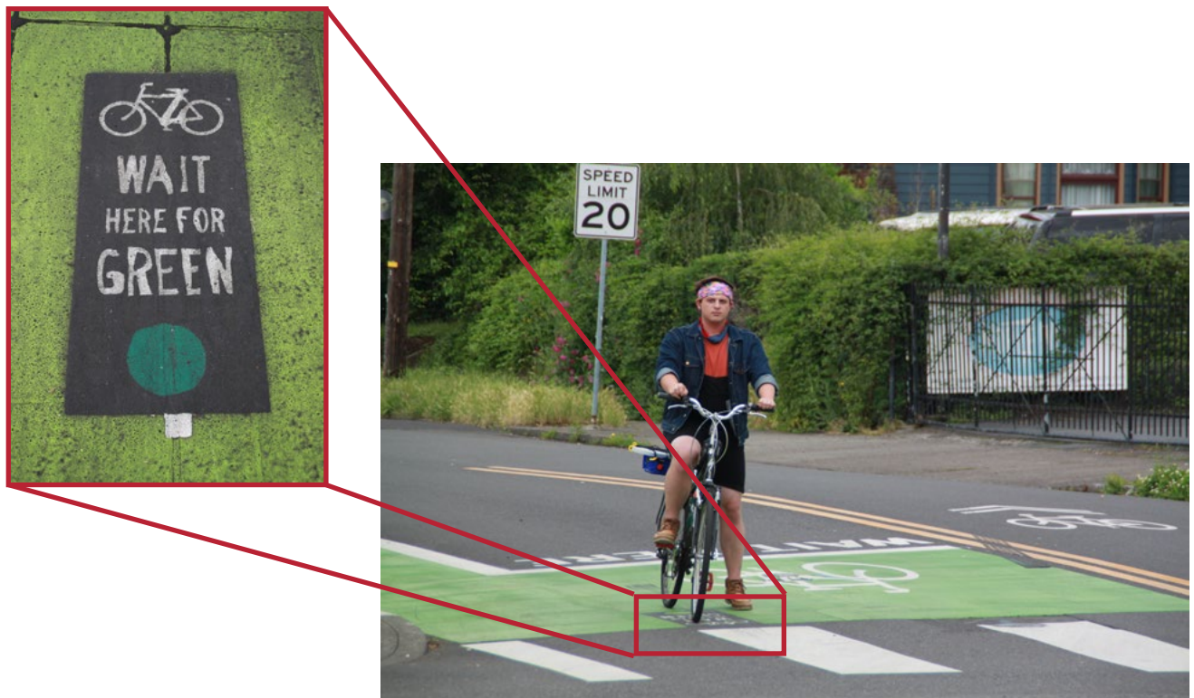
Research found that this modified pavement detector marking was more intuitive to understand by people biking
