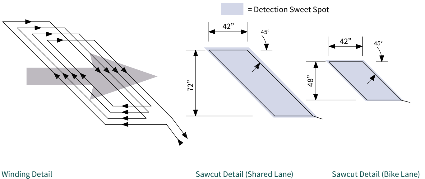
Parallelogram Loop Detector Configuration
