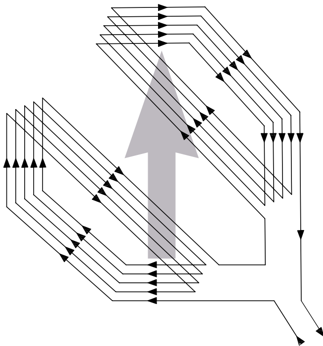
Type D Loop Detector Configuration
