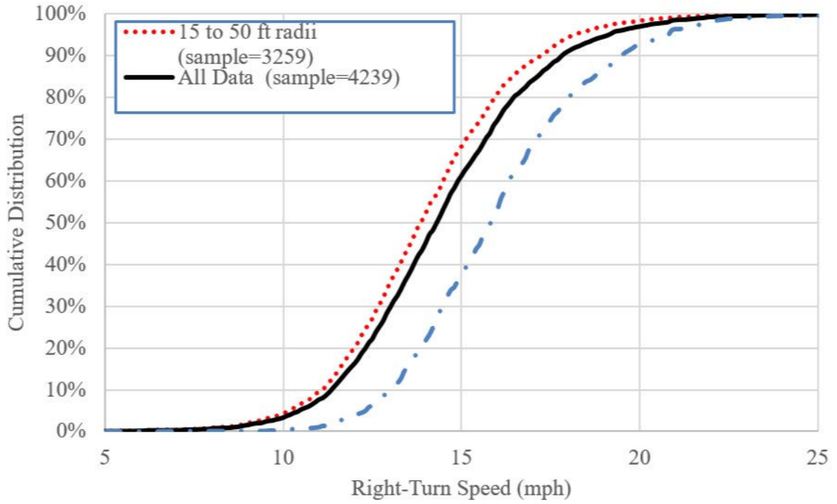
Figure 50. Graph. Passenger car right-turn speed distribution for observed field data.
