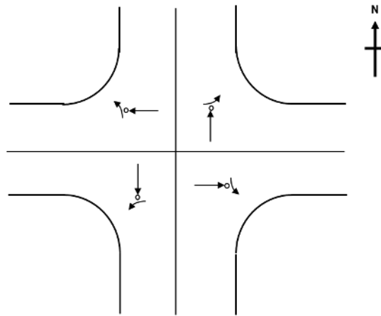
Figure 14. Sketch. Crash assignments to corners based on crash characteristics: right-angle, through and left, passenger's side impacted or same-direction sideswipe, through and left.
