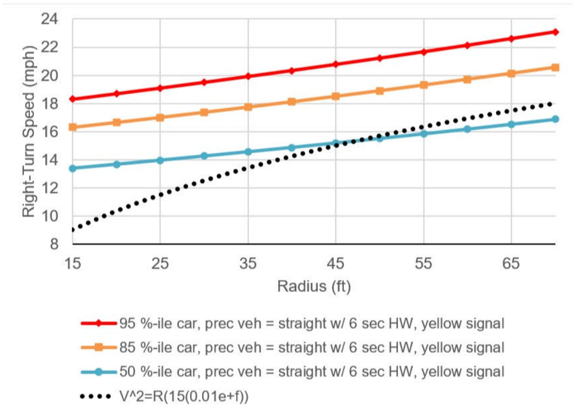
Figure 49. Graph. Comparison of predicted 50th, 85th, and 95th percentile right-turn speeds for stated conditions with calculated speed using radius of curvature equation.
