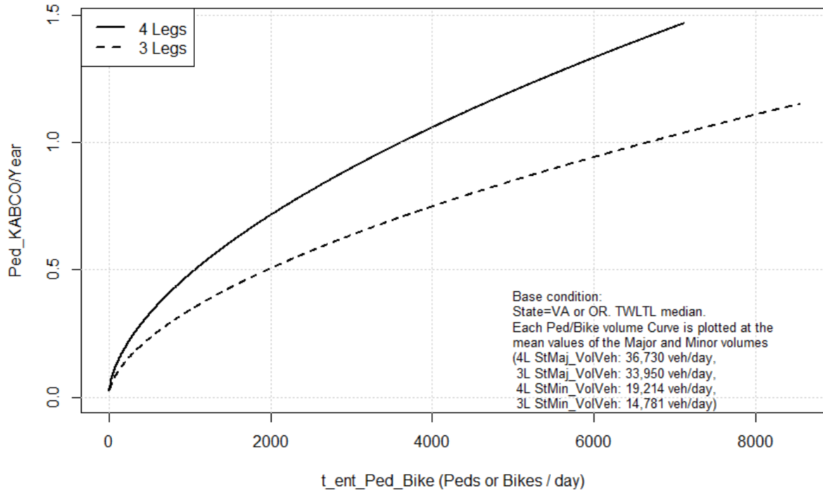
Figure 38. Graph. Ped_KABCO crash model predictions versus pedestrian/bicycle volumes by number of legs.
