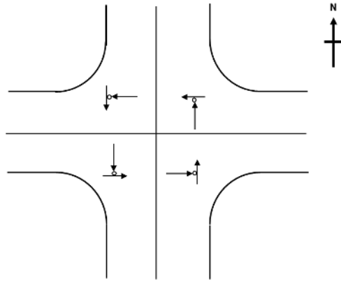
Figure 10. Sketch. Crash assignments to corners based on crash characteristics: right-angle, two throughs, driver's side impacted.
