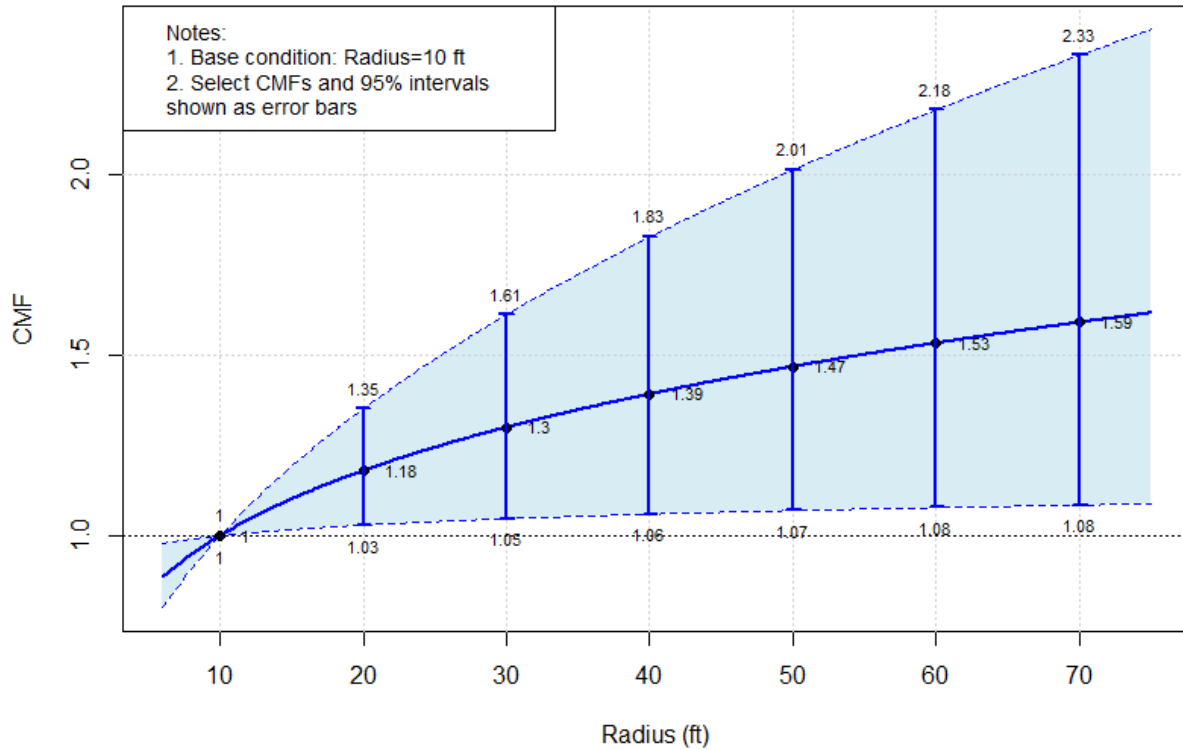
Figure 26. Graph. Corner radius CMF for pedestrian crashes based on Virginia model.
