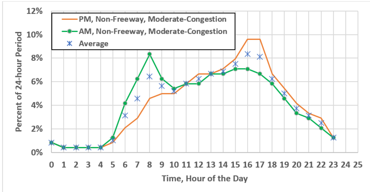
Figure 16. Graph. Daily vehicle distribution used for adjusting vehicle counts.
