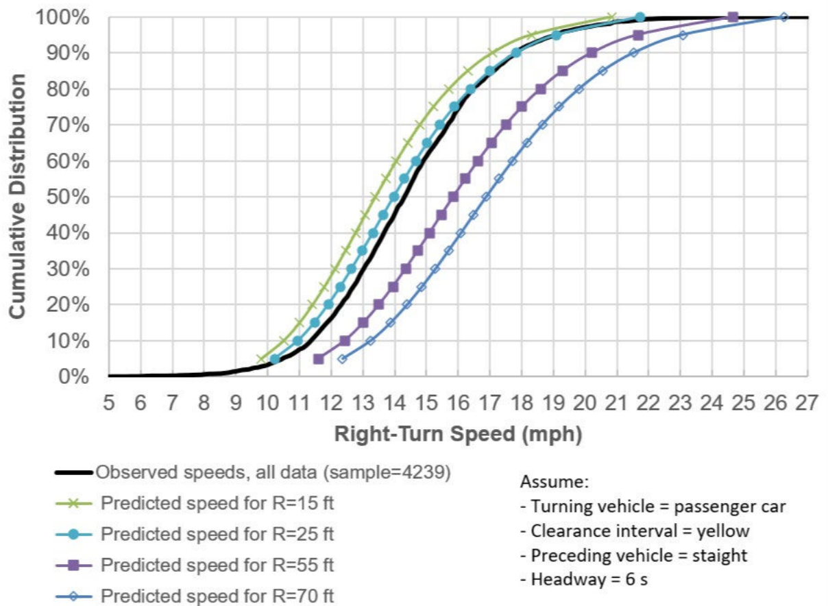
Figure 51. Graph. Passenger car right-turn speed distribution for a sample of corner radius values using prediction equation.
