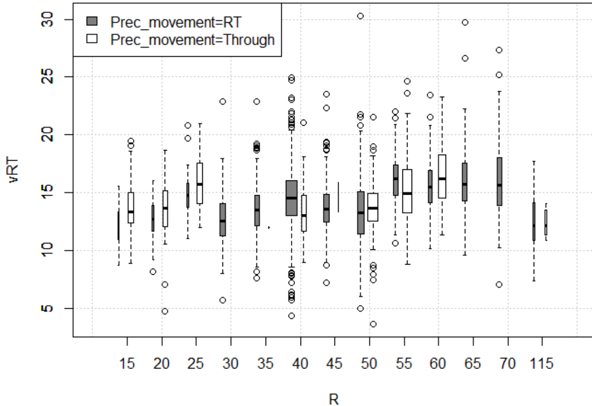
Figure 44. Graph. Speeds of right-turn vehicles by movement of preceding vehicle and radius.
