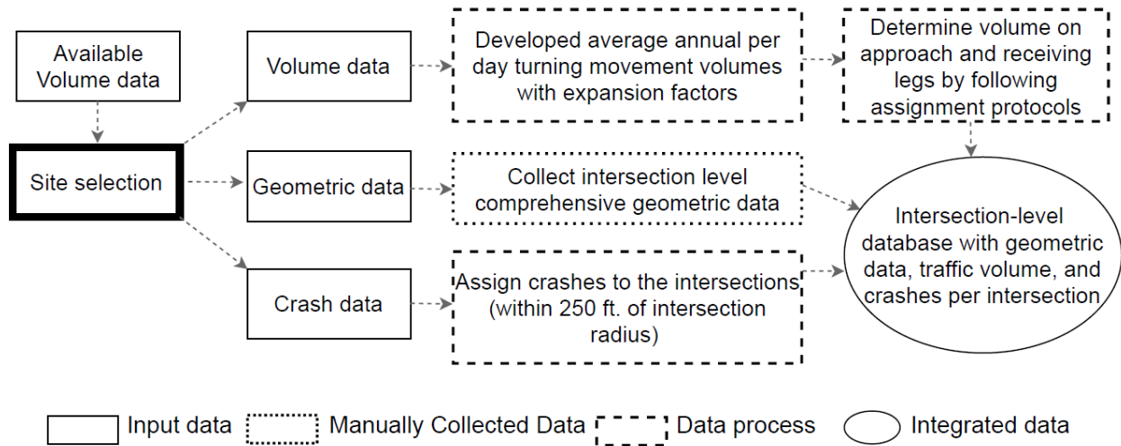
Figure 31. Flowchart. Intersection-level data preparation.
