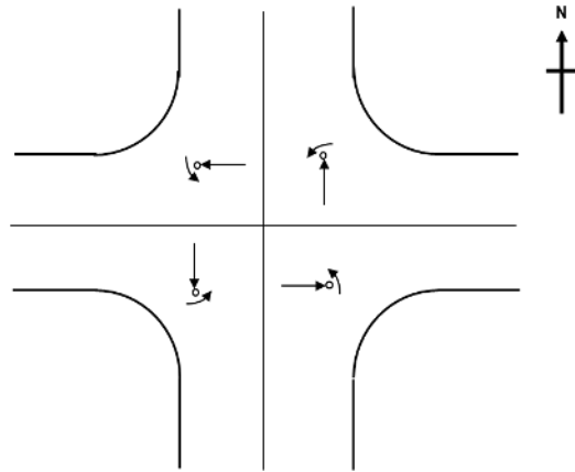
Figure 13. Sketch. Crash assignments to corners based on crash characteristics: right-angle, through and left, driver's side impacted.
