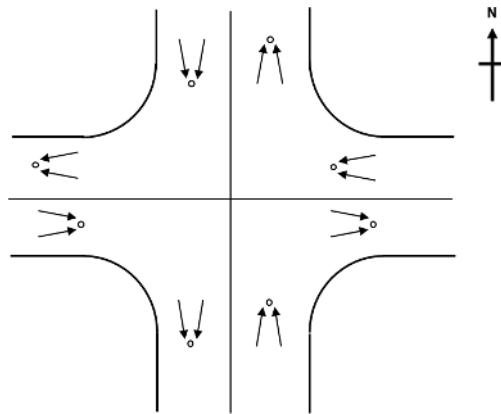
Figure 11. Sketch. Crash assignments to corners based on crash characteristics: same-direction sideswipe, two throughs.
