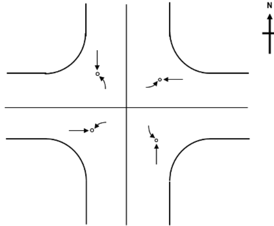
Figure 15. Sketch. Crash assignments to corners based on crash characteristics: left-turn opposed.
