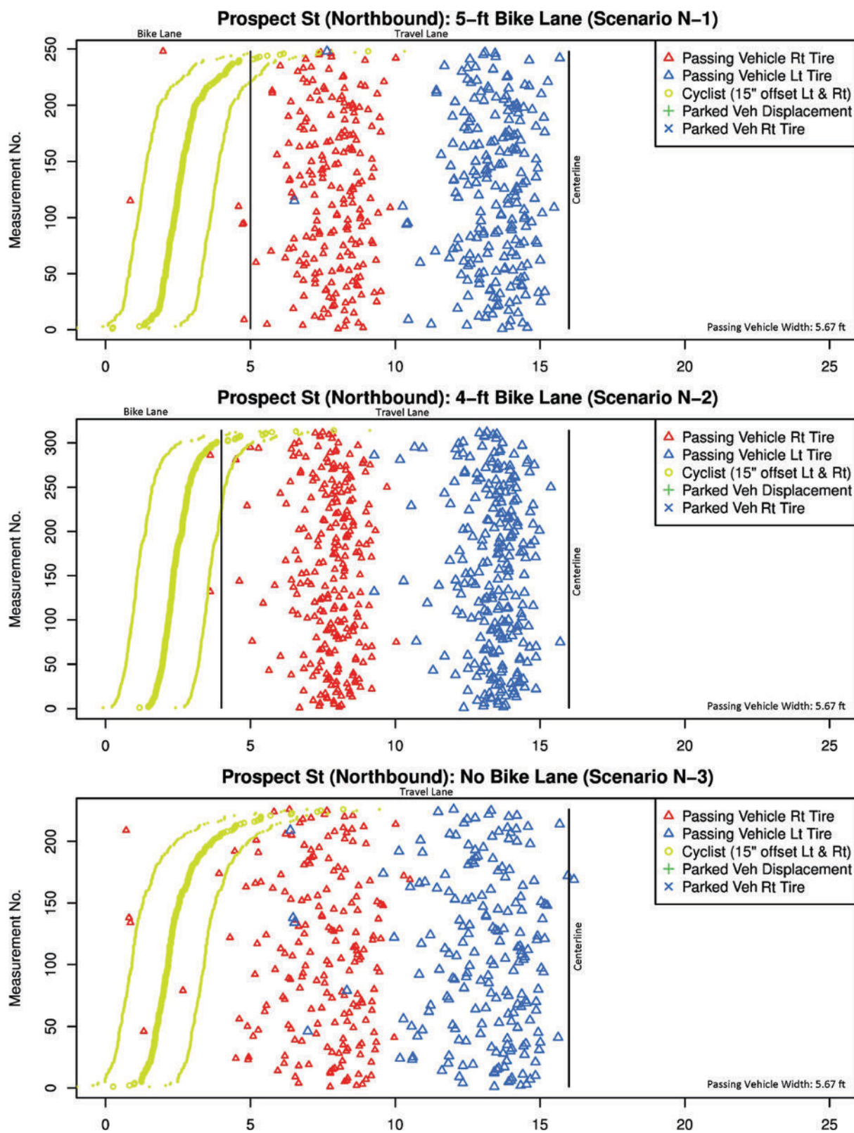
Figure 17. Measurements taken on Prospect Street (northbound) in Cambridge (assumed 5.67-ft width for passing vehicle).
