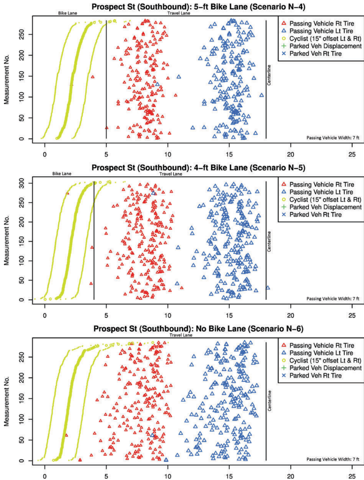
Figure 13. Measurements taken on Prospect Street (southbound) in Cambridge (assumed 7-ft width for passing vehicle).
