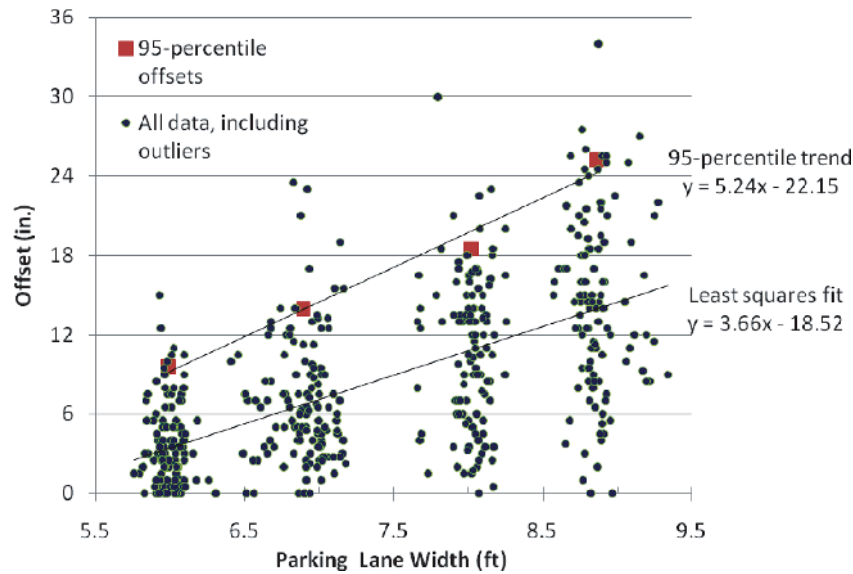
FIGURE 1 Parking offset versus lane width.
