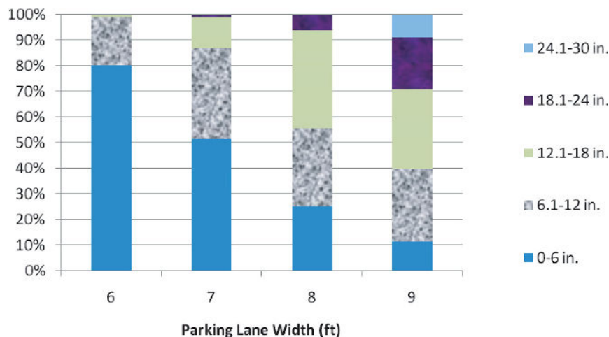
FIGURE 3 Relative frequency distribution of parking offset by parking lane width.
