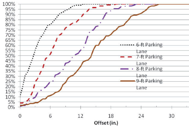
FIGURE 2 Cumulative distribution of parking offset by parking lane width.
