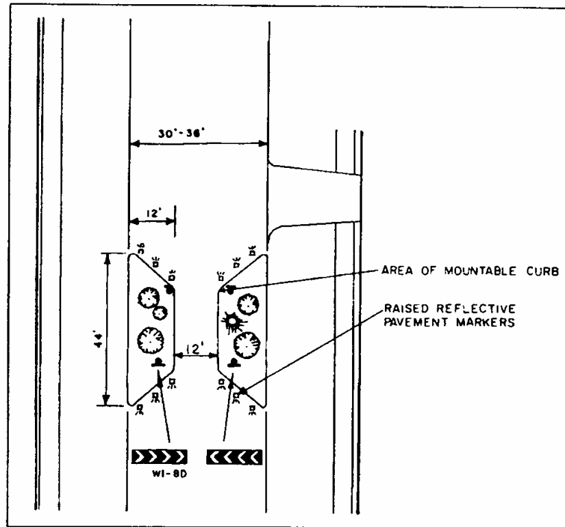
Figure 9. Parallel Choker (13)
